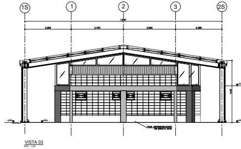
VISTA 03 4502.1150
